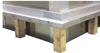
Pallet Forms placed on Riser Forms.
